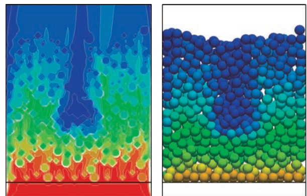
Temperature evolution in non-uniform packed bed.
