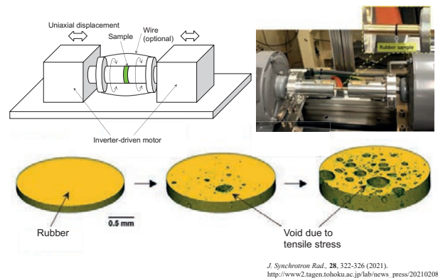
Real-time 4D observation of rubber tensile fracture process (10 ms temporal resolution)
