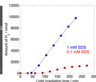
SEM image of Pt-deposited pi-conjugated organic nanofibers and H 2 generation under visible light irradiation.
