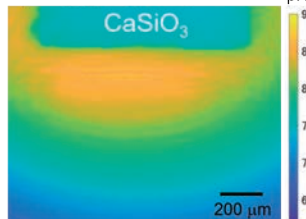
pH imaging during leaching of silicate
