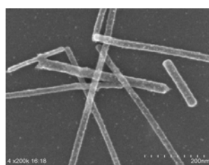
SEM image of Pt-deposited pi-conjugated organic nanofibers and H 2 generation under visible light irradiation.
