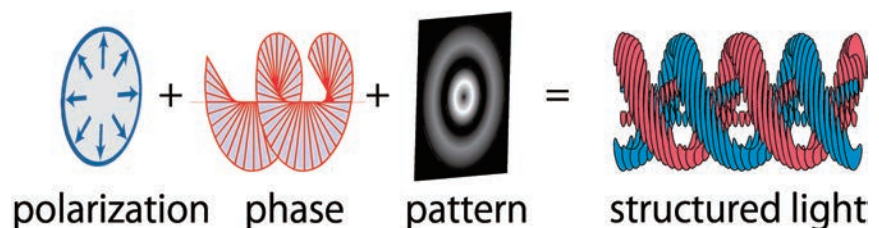
Structured light reveals synergetic aspects of polarization, phase and pattern of light beams.
