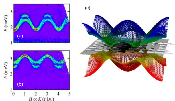
(a,b) Observed dispersions of triplons along H (or K ) with the K (or H ) integrated around (a) K (or H ) = 0, or (b) K (or H ) = -\pi . The integration range is |\Delta K| (or |\Delta H| ) < 0.1 . (c) Calculated modeled dispersions with the fictitious magnetic field shown by the arrows.
