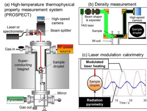
High-temperature thermophysical property measurement system (PROSPECT)
