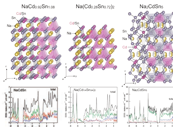
新規 Na-Cd-Sn 系金属間化合物の結晶構造と電子状態密度 New ternary intermetallic compounds in the Na-Cd-Sn system found in 2021; the crystal structures and calculated density of electronic states.
