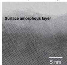
Structural analysis of silicate by TEM
