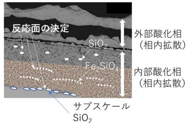
Figure. Analysis of reaction mechanism and control of high temperature reaction
