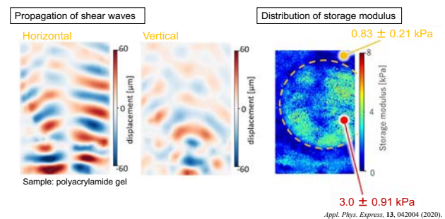
X-ray elastography by visualizing propagating shear waves
