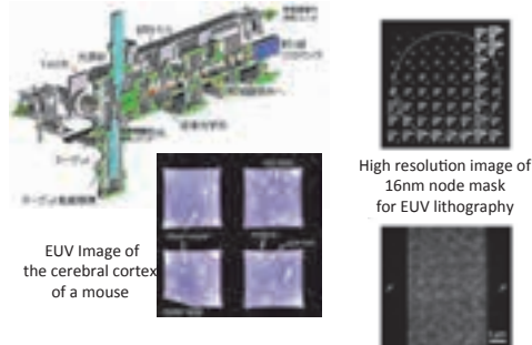
Fig.2 Transmission X-ray Multilayer Mirror Microscope (TXM 3 ) T. Ejima, M. Toyoda, T. Hatano, M. Yanagihara & M. Yamamoto
