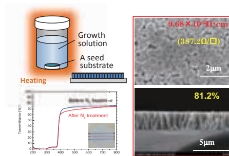
溶液プロセスによる配向性透明導電性薄膜の調製 Preparation of oriented transparent conductive thin film by solution process
