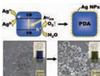
Polydiacetylene (core) - silver (shell) hybridized nanocrystals fabricated by visible-light-driven photocatalytic reduction method.
