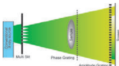
Configuration of X-ray Phase Imaging —X-ray Talbot-Lau interferometer—
