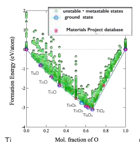
Ground state analysis using Genetic Algorithm
