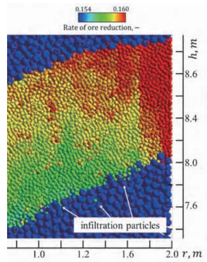
Distribution of reaction degree calculated by particle tracking technique
