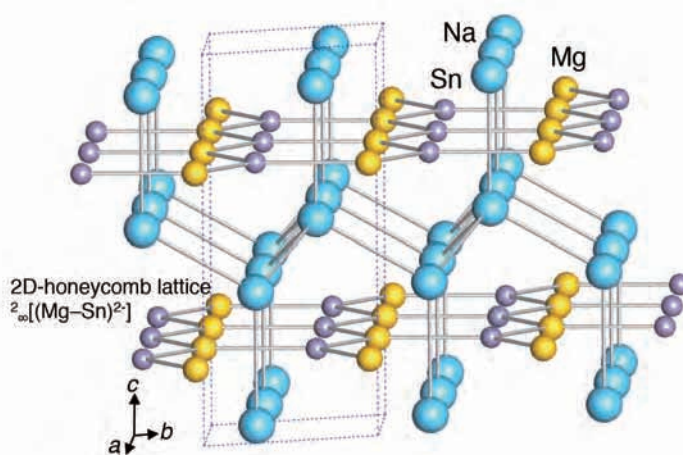
Schematic drawing of the crystal structure of Na 2 MgSn.
