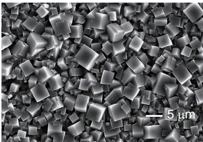
Scanning electron micrograph of \text{NaB}_5\text{C} bulk ceramics prepared at 800°C.
