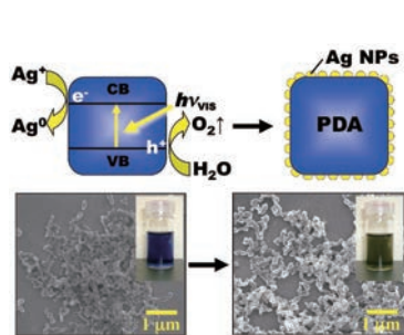
Polydiacetylene (core) - silver (shell) hybridized nanocrystals fabricated by visible-light-driven photocatalytic reduction method.
