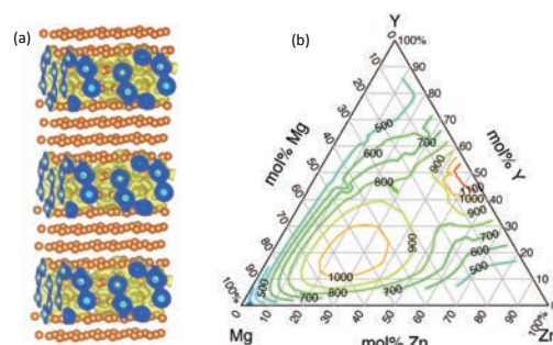
(a) Calculated charge density of the LPSO-type Mg alloys and (b) Spinodal temperature of the Mg-Zn-Y system based on the cluster variation method
