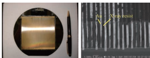
X-ray Optical Element —High Aspect-Ratio Gold Grating—
