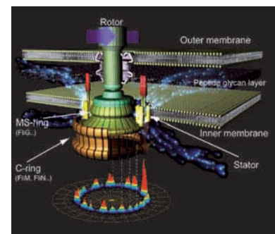
Bacteria flagellar motor
