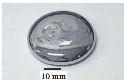
High purity Fe (>99.9998 mass%), the highest level in the world, refined by a novel purification method
