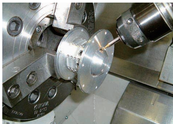
Multi-tasking machine
