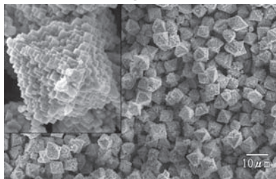
Na 0.5 K 0.5 NbO 3 for lead-free piezoelectric devices
