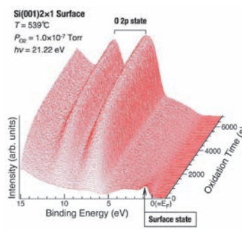
Fig.1. Time evolution of valence band photoelectron spectra taken in situ during oxidizing Si(001)2 × 1 surface with O 2 .
