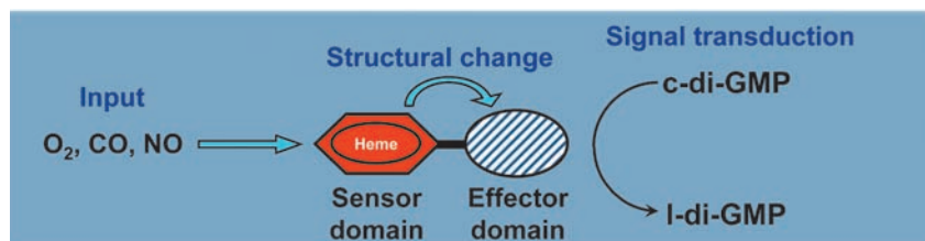
Fig. 1: Gas-sensing of Ec DOS
