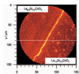
Nanohetero-interface design for fast oxygen reduction reaction (Bright part is the fast reaction zone).
