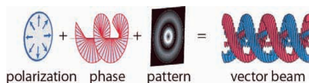
The vector beam under study shows a synegetic aspect of polarization, phase and pattern of a light beam.
