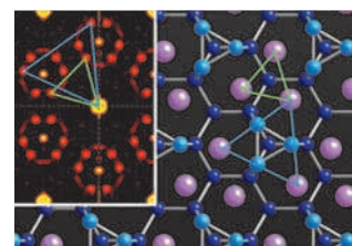
Fig.2. Patterson map (inset) and Structure model of Si(111)√3x√3-Ag surface: Ag (pink spheres) and Si (blue spheres) obtained by Weissenberg RHEED.
