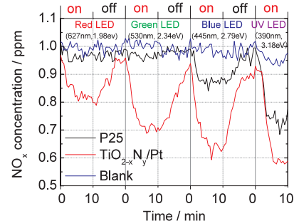
LEDランプによる可視光応答性光触媒の評価 Characterization of Visible Light Responsive Photocatalysts by LED Lights Irradiations
