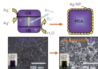
Polydiacetylene (core) - silver (shell) hybridized nanocrystals fabricated by visible-light-driven photocatalytic reduction method.
