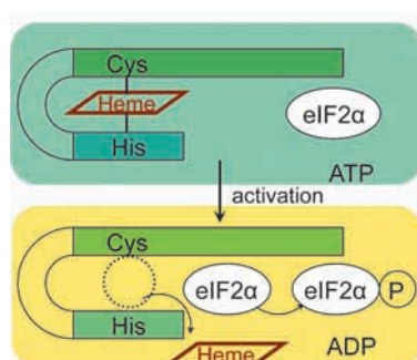
Fig. 2: Heme-sensing of HRI.
